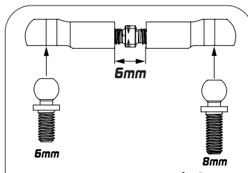
From Servo Link
