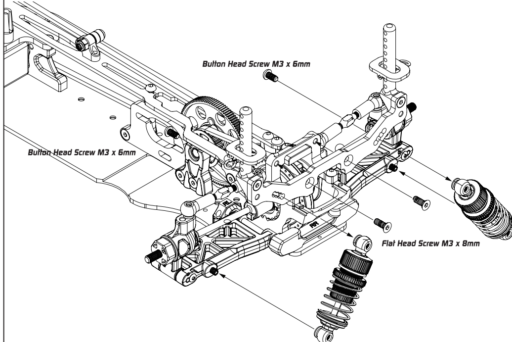
Flat Head Screw M3 x 8mm
