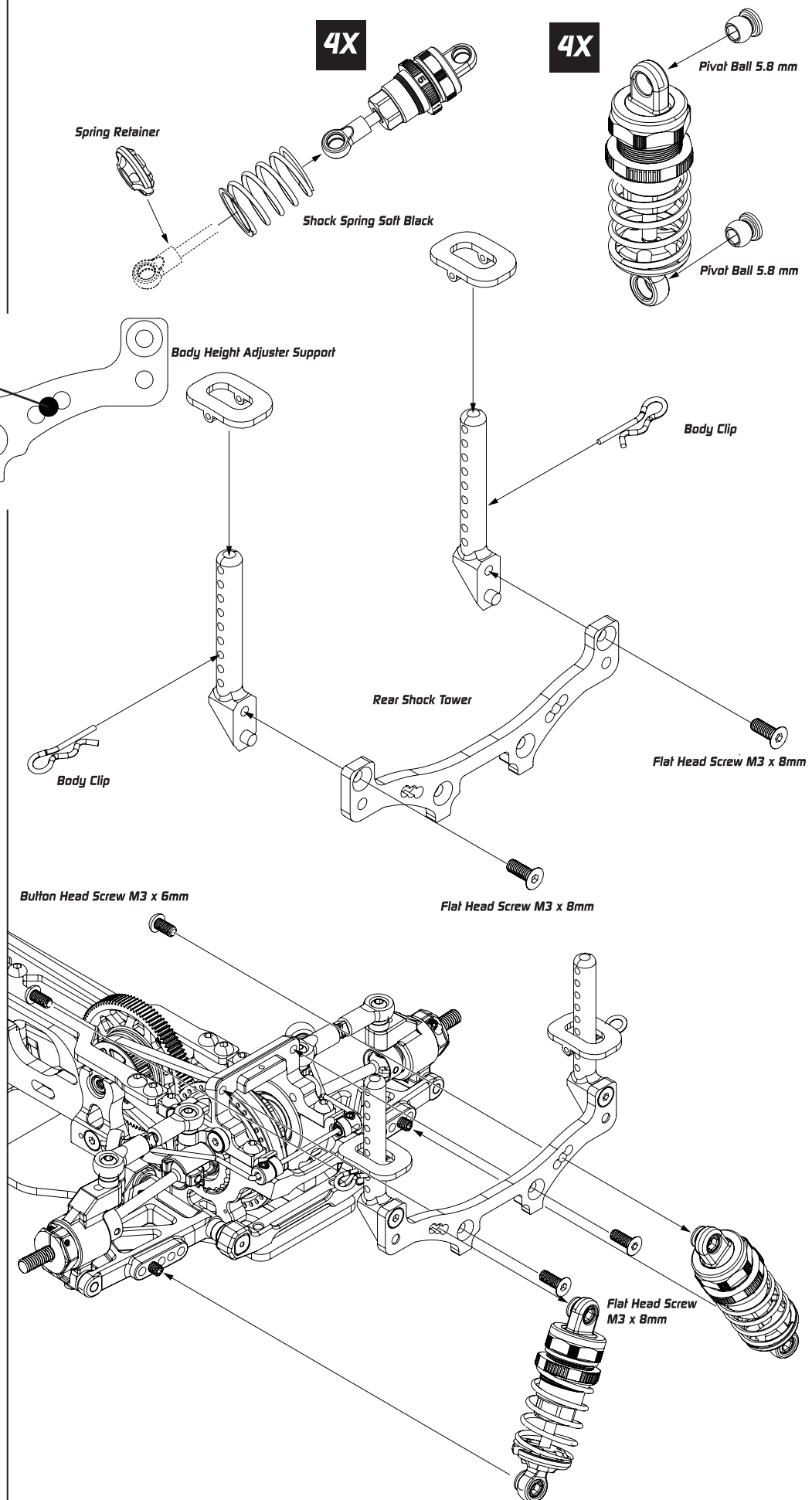
Body Height Adjuster Support XP-10001
