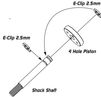
E-Clip 2.5mm
